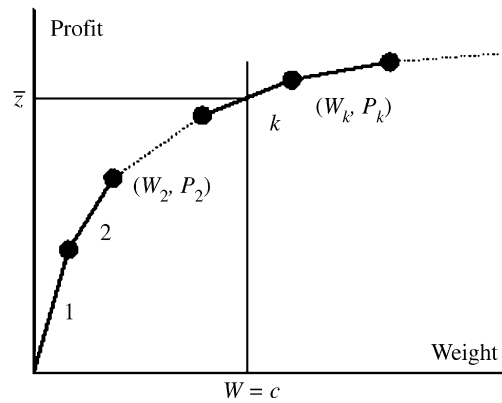
Fig. 1. Solution of SMKP( \lambda ).
